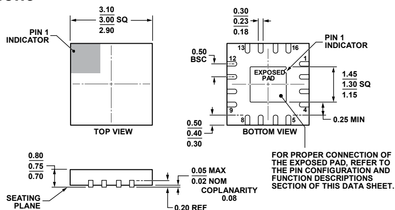
Figure 61. 16-Lead Lead Frame Chip Scale Package [LFCSP_WQ] 3 mm × 3 mm Body, Very Very Thin Quad (CP-16-21)
