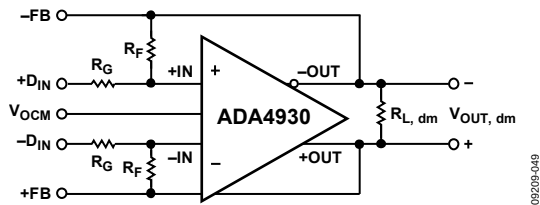
Figure 42. Circuit Definitions
