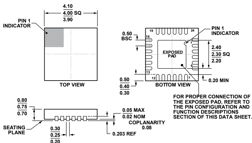
Figure 62. 24-Lead Lead Frame Chip Scale Package [LFCSP_WQ] 4 mm × 4 mm Body, Very Very Thin Quad (CP-24-14)
