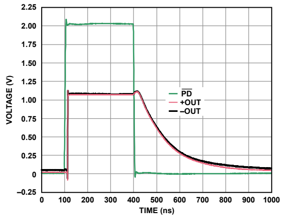
Figure 37. \overline{PD} Response vs. Time
